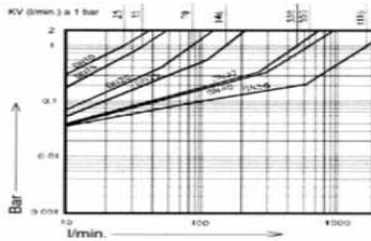
With water at 20°C (valve with spring)
